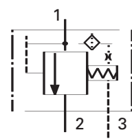
DPS2-**-V Spool, normally closed
