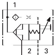
DPS2-**-B Poppet, vent to open, normally closed
