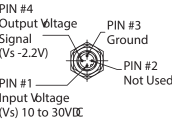
Connector Detail
