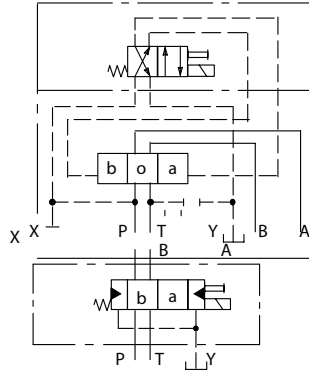
Spring Offset, End-to-End, Opposite Hand, DG5V-10-*AL
