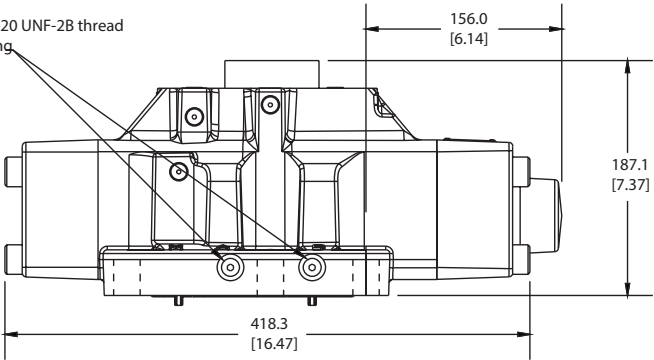
DG3V-10-*A-11 Series
