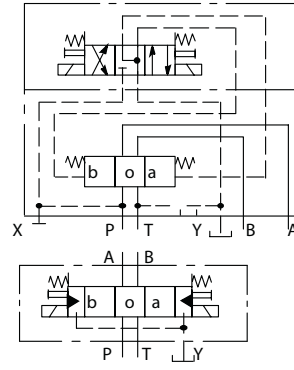
Spring Centered, DG5V-10-*C
