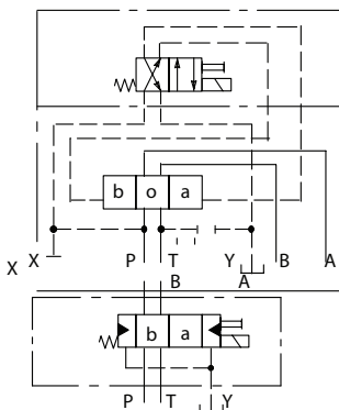
Spring Offset, End-to-End, Opposite Hand , DG5V-8-*A L
