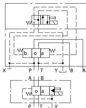
Spring Offset, End-to-Center, Opposite Hand DG5V-8-*BL
