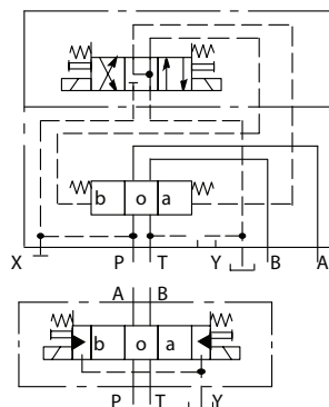
Spring Centered , DG5V-8-*C
