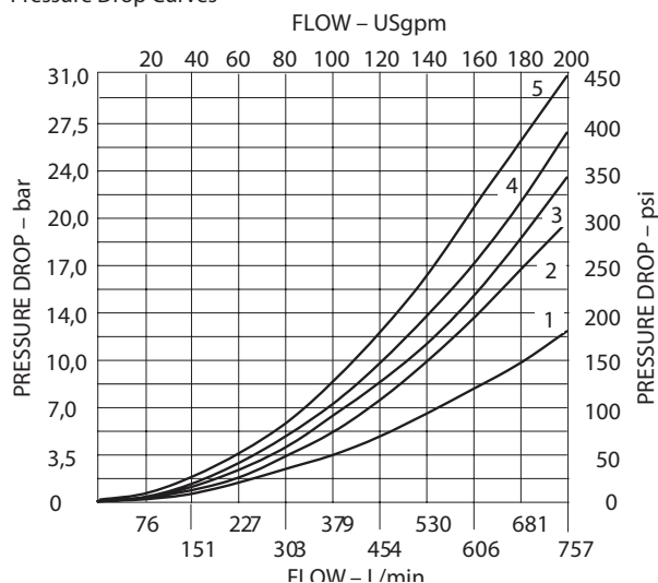
Pressure Drop Curves
