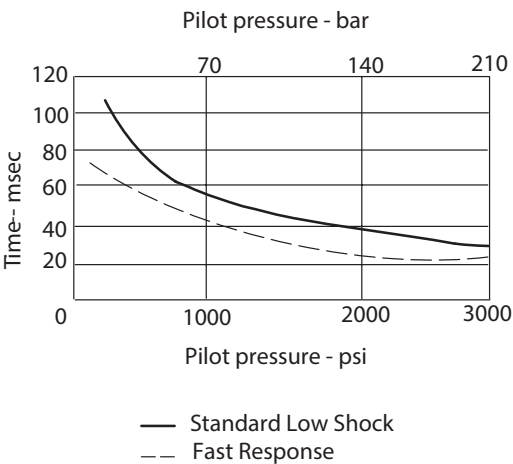
Centering Times for Pressure Centered Valves @ Rated Pressure (A to P or B to P)
