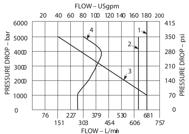
Malfunction Flow Curves
