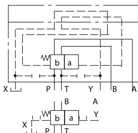
Spring Offset, End-to-End, Opposite Hand, DG3V-8-*AL
