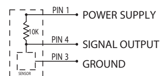
Output Circuit Wiring Instruction:
