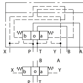
Spring Centered, DG3V-8-*C
