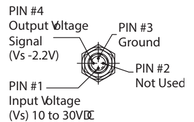
Connector Detail
