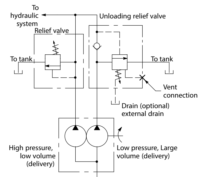
Double Pump Circuit
