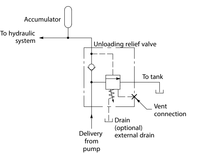
Accumulator Circuit
