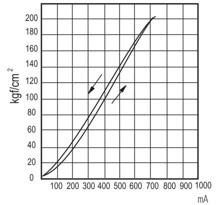
EBG-10(H)
