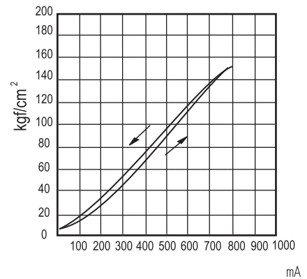
EBG-10(C)
