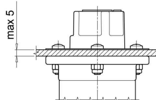
Internal mount
