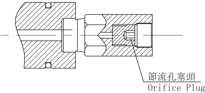
滿油閥 導壓口接頭 Pre-fill valves pilot port adaptor
