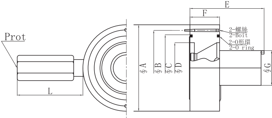
滿油閥 Pre-fill valves
