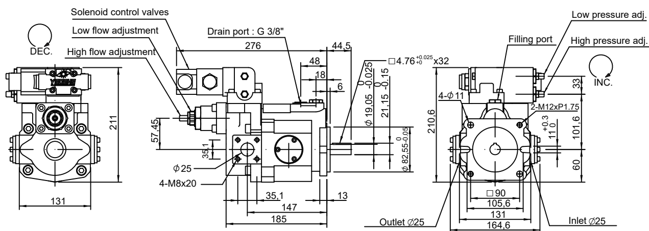
V15FG, V18FG Electric 2-stage pressure control &amp; Flow control + Remote
