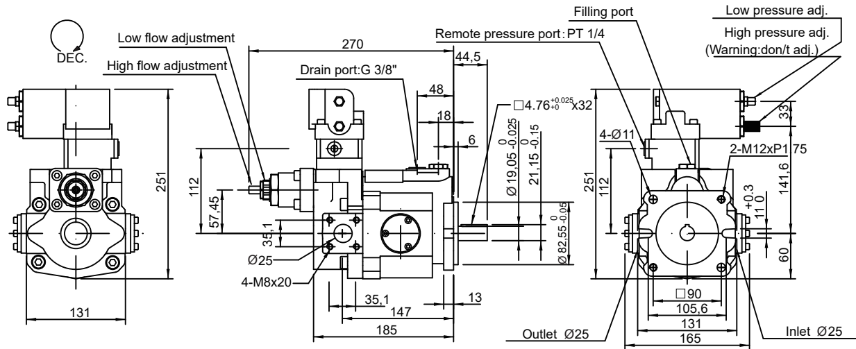
V15CG, V18CG 2-stage pressure &amp; Flow control + Remote
