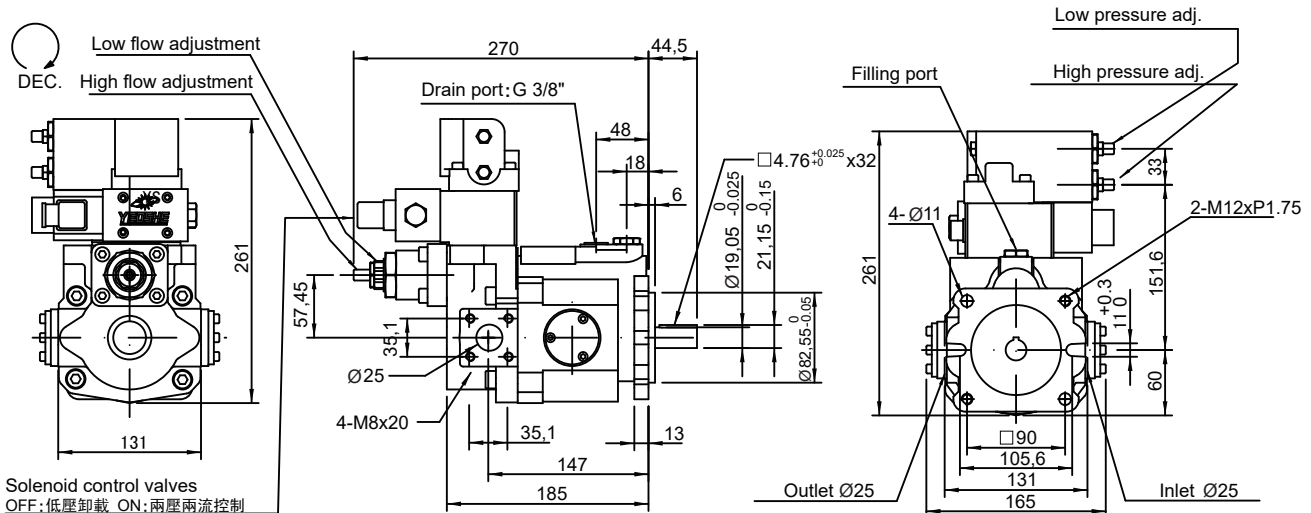
V15CR, V18CR 2-stage pressure &amp; Flow control + Low tension unloading
