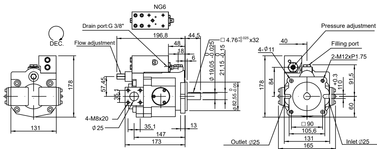
V15GM, V18GM Remote pressure compensator with NG6 interface
