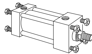
TV23 Both ends extended tie rod ISO MX1
